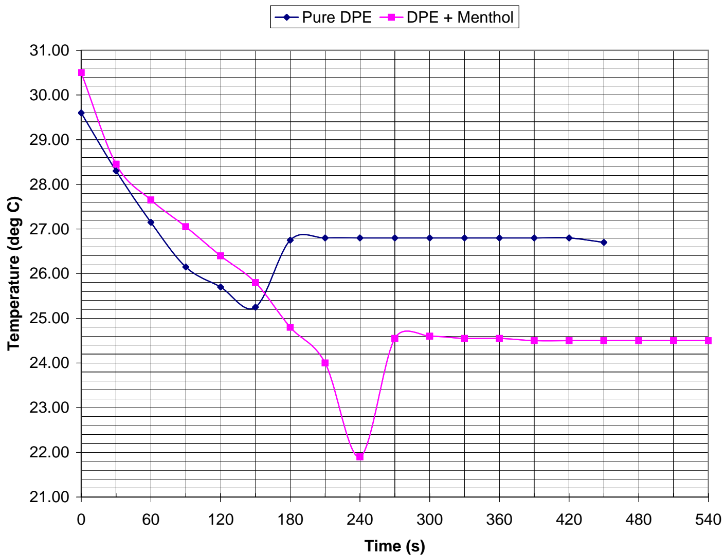
Freezing Point Depression of Diphenyl Ether by Menthol
